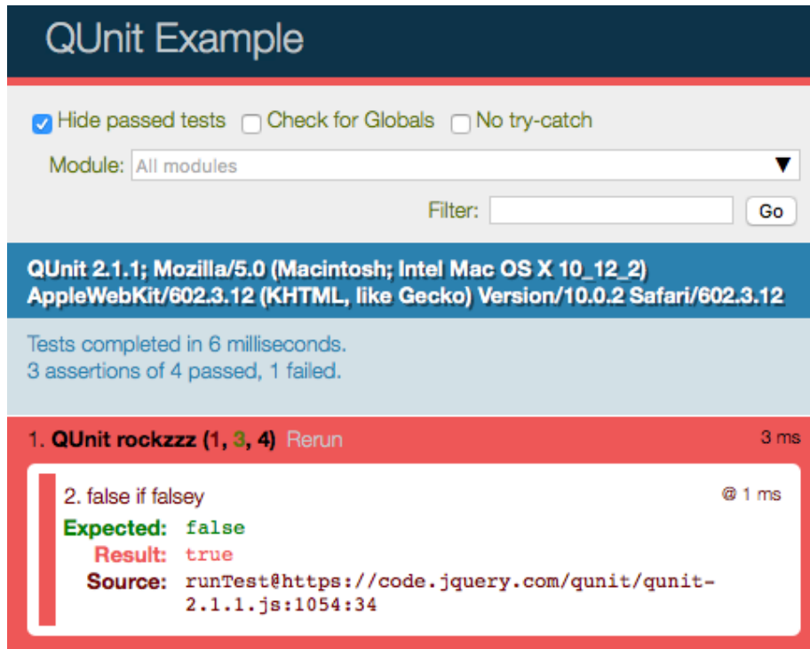
Figure 3: Qunit failure example
